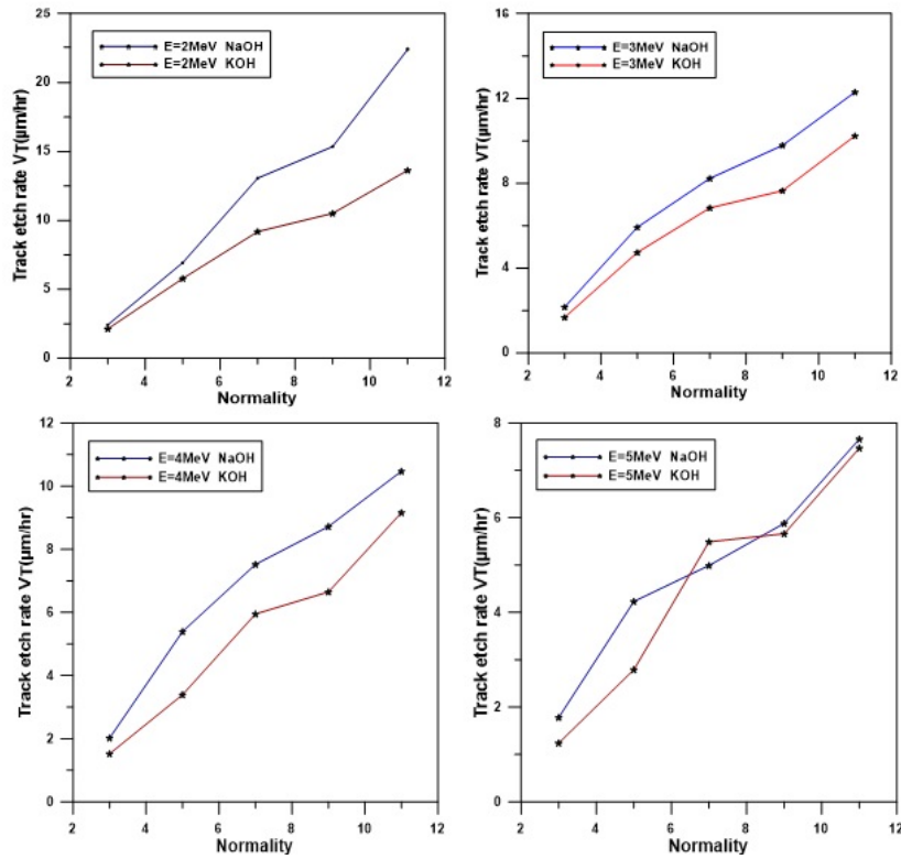
Figure 2. The Track etching rate V_T as a function of KOH and NaOH etchants normalities for alpha energies (2, 3, 4, 5) MeV.
