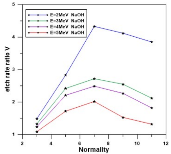
Figure 4. The etch rates ratio V as a function of normality of the NaOH solution at different alpha energies (2, 3, 4, 5) MeV.
