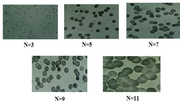
Figure 5. Alpha particles tracks of energy 3 MeV in CR-39 detector.
