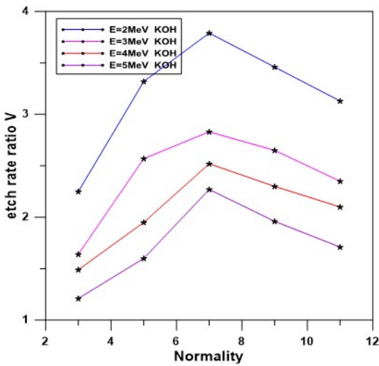
Figure 3. The etch rate ratio ( V ) as a function of normality of the KOH solution at different alpha energies (2, 3, 4, 5) MeV.
